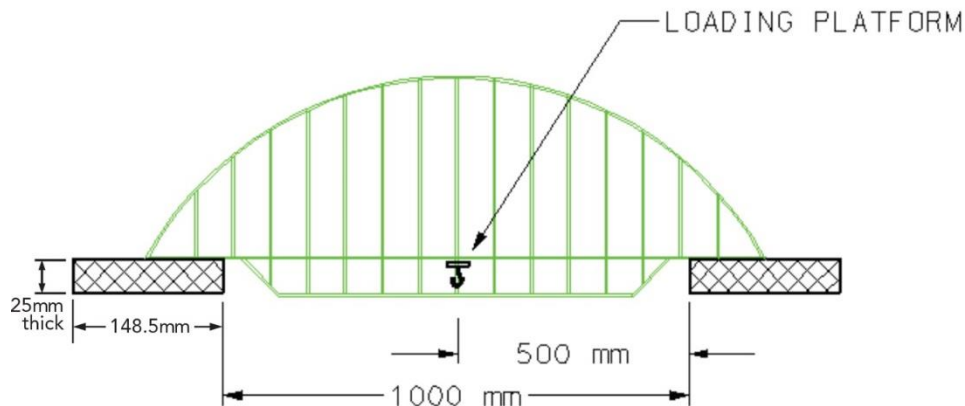
Figure 7: Location of Loading Platform
