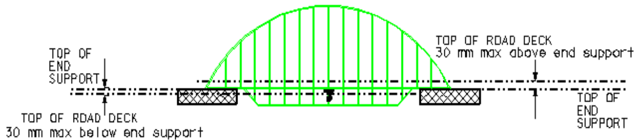
Figure 4: Bridge Deck Vertical Position
