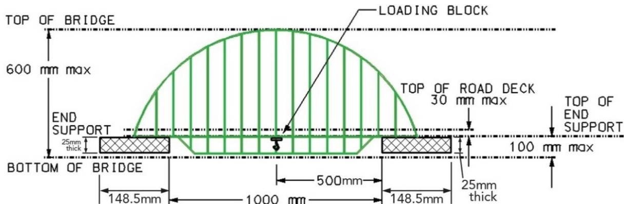
Figure 1: Overall Bridge Dimensions
