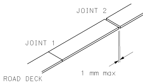
Figure 3: Joints Across Road Deck
