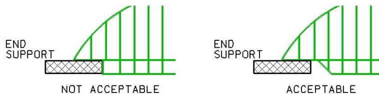
Figure 5: Use of End Support
